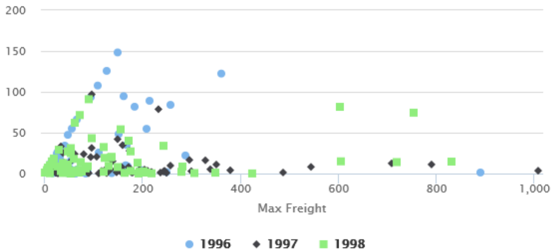
Figure 17-25 Scatter chart
