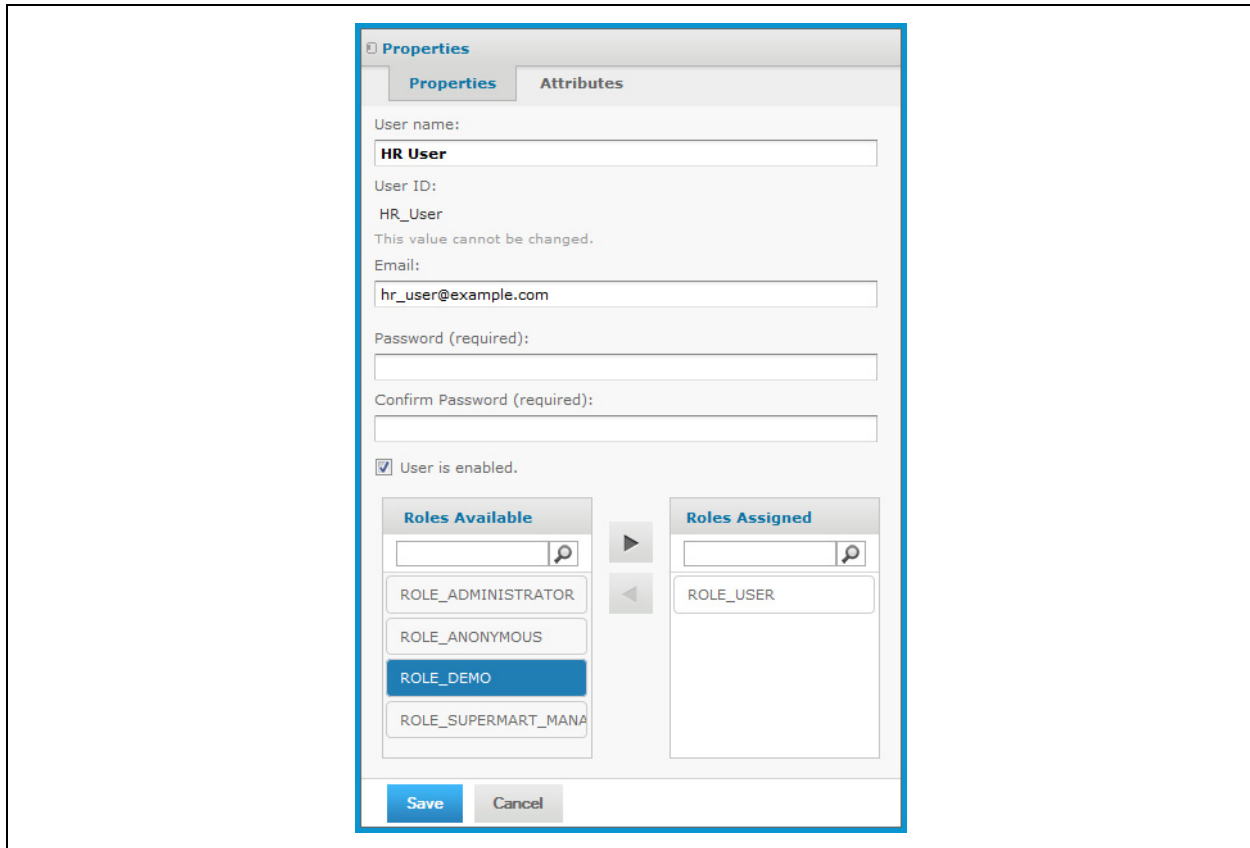
Figure 2-7 Editing the Properties of a User
