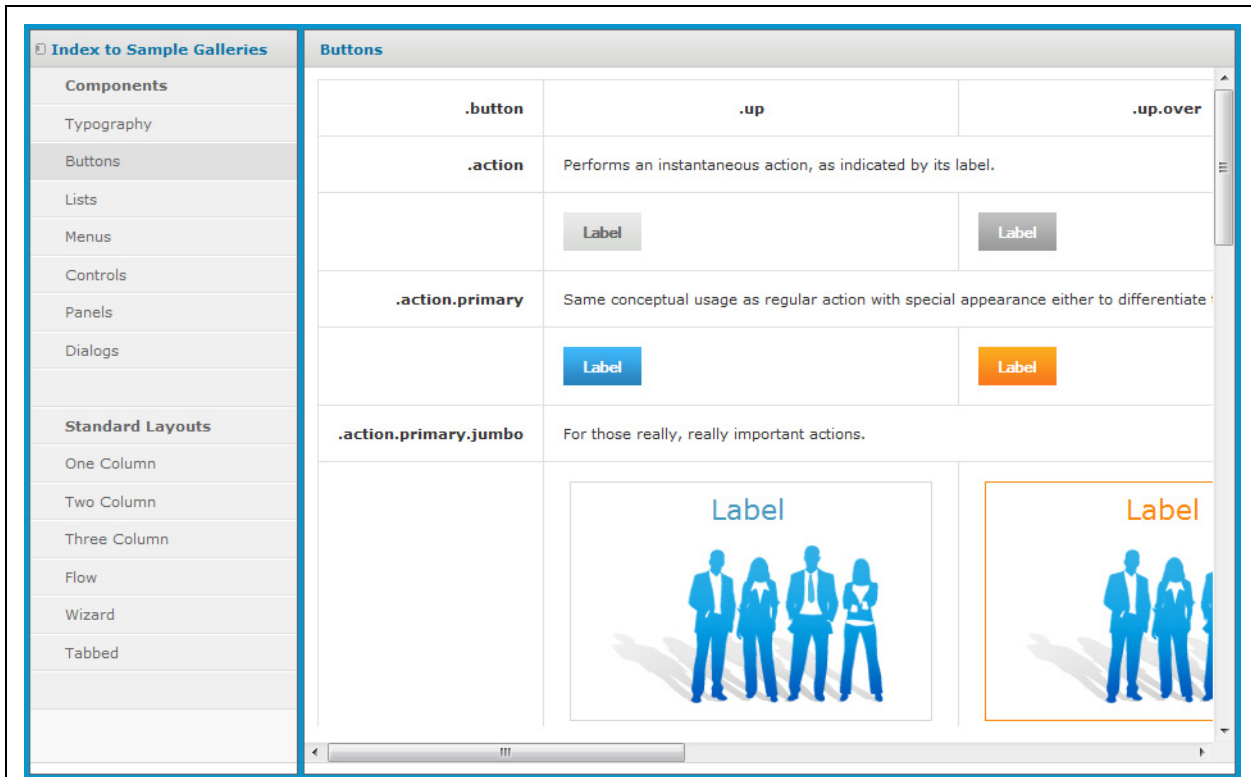
Figure 5-8 All Possible Button Components in the Sample Galleries
