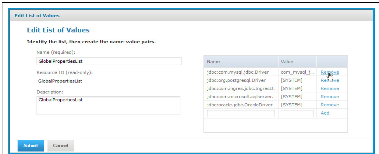
Figure 4-7 Removing an Uploaded JDBC Driver
