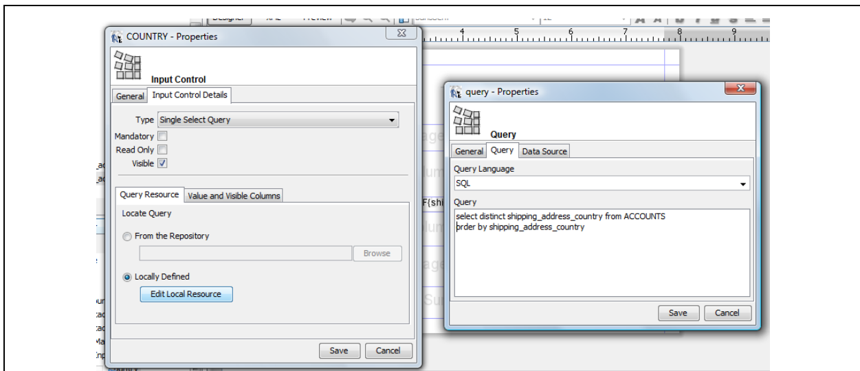
Figure 4-32 Creating the COUNTRY Input Control
