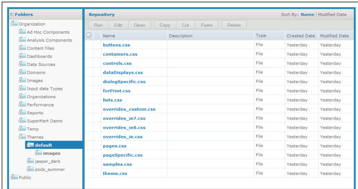
Figure 5-5 Organization Themes Seen by Organization Admin
