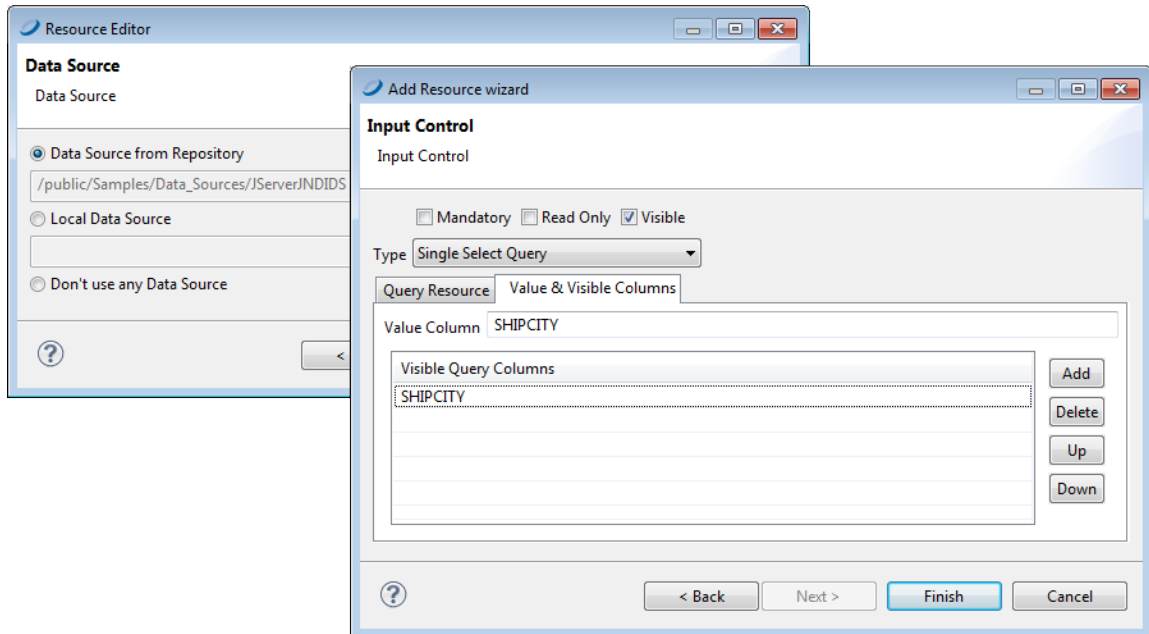
Figure 5-19 City Control Value and Visible Columns
