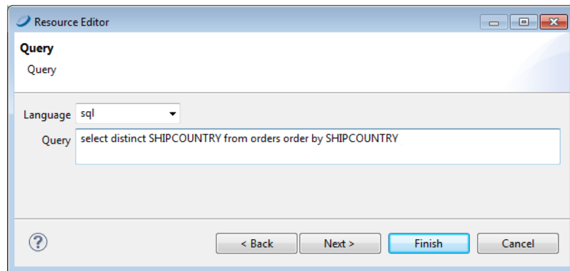
Figure 5-16 Query for the Country Input Control
