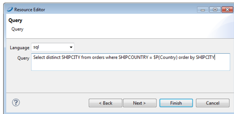
Figure 5-18 Query Using Country to Select Cities
